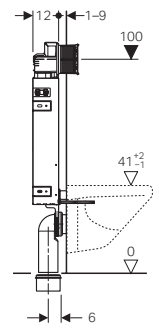
Kombifix element with Sigma concealed cistern, thickness 120mm, height 1080mm
